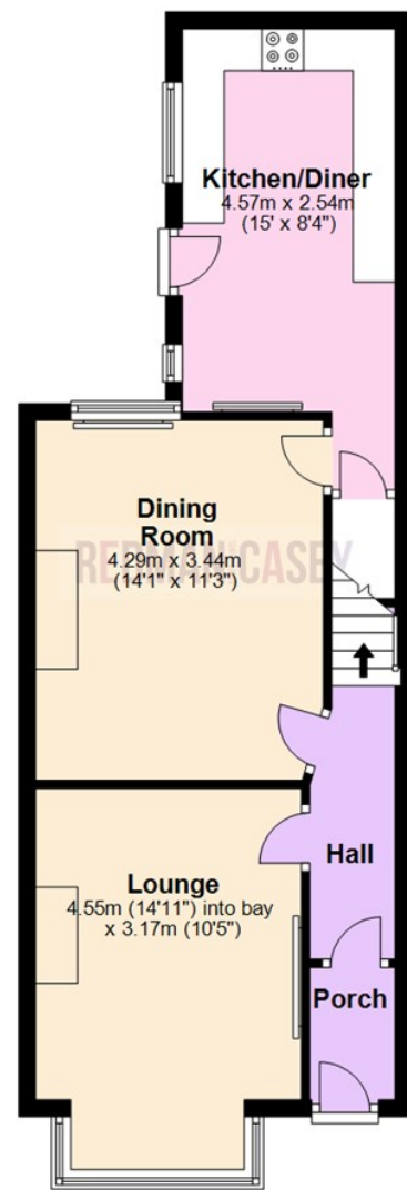
Ground Floor Approx. 47.5 sq. metres (511.4 sq. feet)
